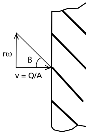
Figure 8. Velocity diagram for rotor radius (r) ideal case
