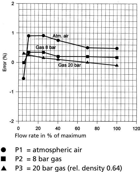
Figure 3. Error of SM-RI turbine meter, 150 mm, 1000 m 3 /h max, as a function of flow rate at three different pressures.
